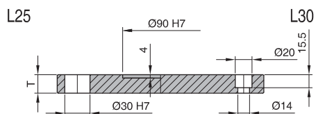
L30/296x346
